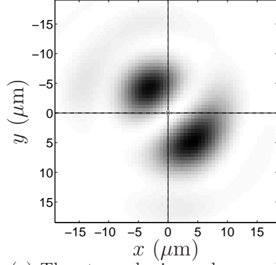
(a) The atmospheric random seed is 3 and the image is frame 2719 of 5120. The value of absolute Strehl is S_A = 0.0014 (-28.7) dB.
