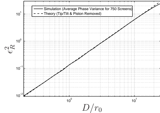
(d) Tip/Tilt-Removed Mean Square Phase (log-log)
