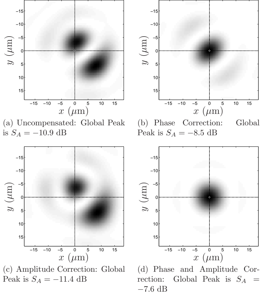
Figure 5.4: Focal plane images for various corrections to the pupil plane field and a uniform turbulence profile of C_n^2 = 2 \times 10^{-17} \text{ m}^{-2/3} . The atmospheric random seed is 3 and the image is frame 2719 of 5120. The scenario is a 100 km path with a 10 m/s uniform crosswind.
