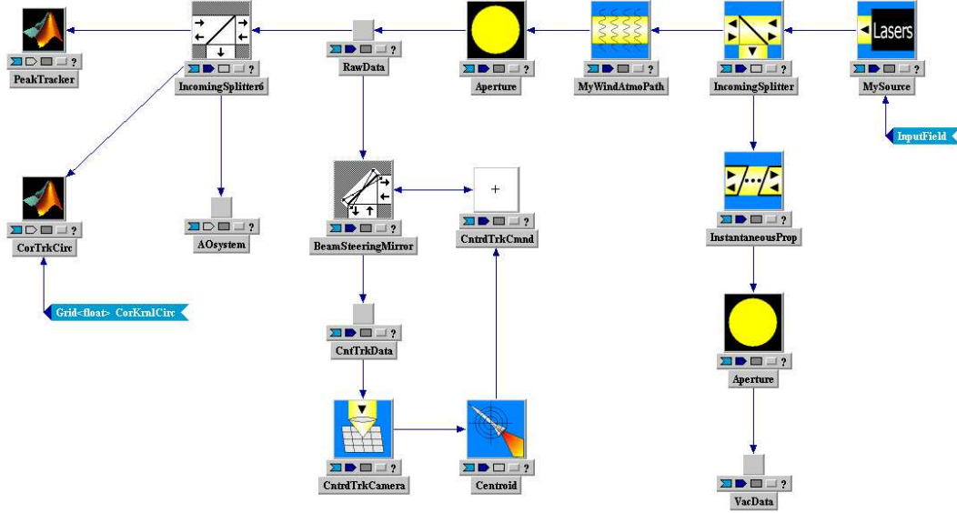
Figure 4.2: The WaveTrain™ model used to generate a wave-optics simulation for studies of deep fade phenomenology and fade mitigation.
