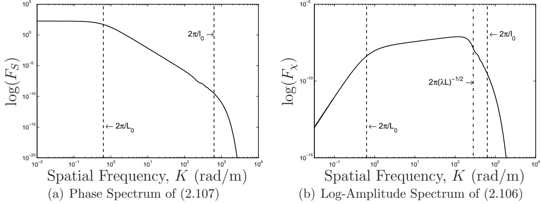
Figure 2.2: PSDs for phase and log-amplitude fluctuations as predicted by Rytov theory for a constant turbulence strength path. Propagation distance is L = 1 km and the wavelength is \lambda = 0.5 \mu\text{m} . The modified von Karman atmospheric PSD was used with L_0 = 10 m and l_0 = 1 cm.
